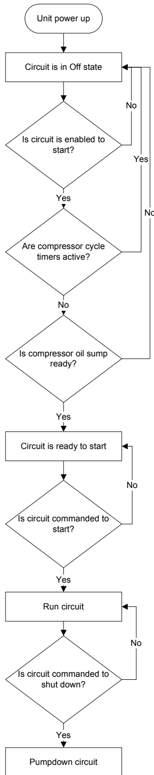
Figure 6, Circuit Sequence of Operation
